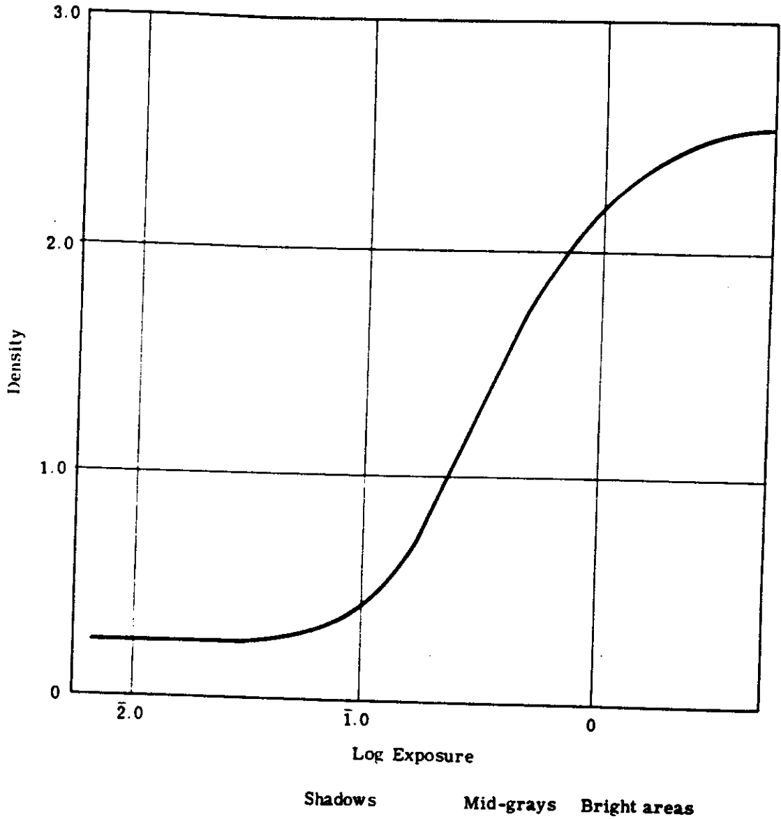
Fig. 6-1 — A general characteristic curve for 3404
